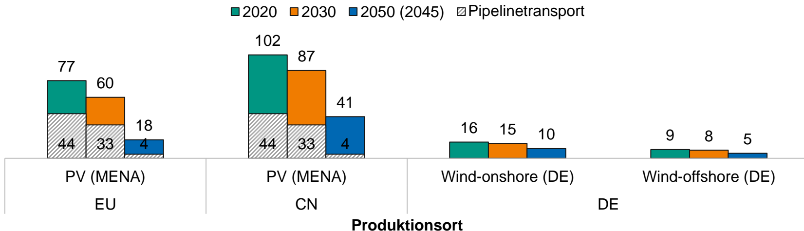
Carbon Footprint grüner H 2 in g CO 2 -eq/kWh
